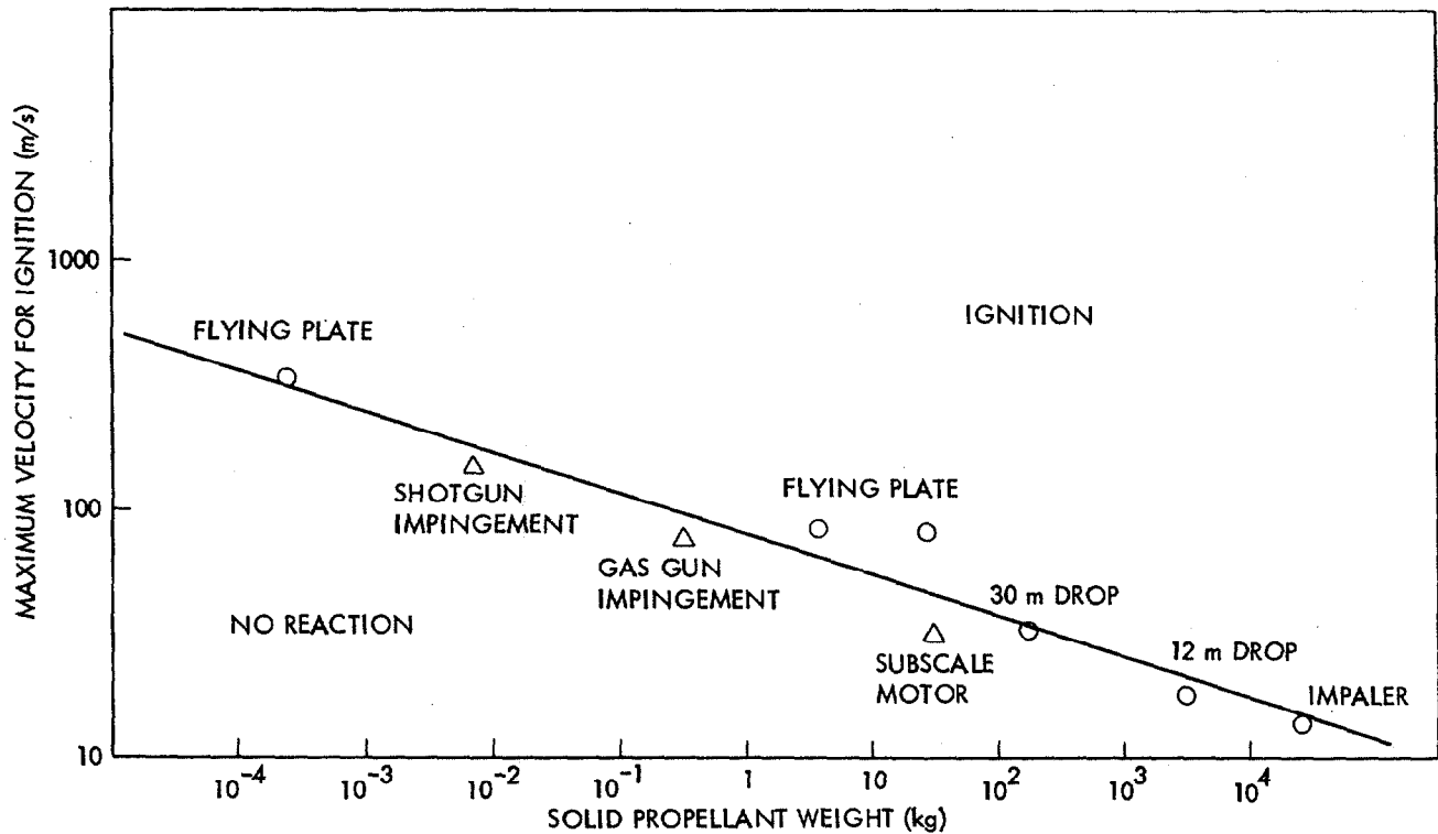
Fig 4 Ignition of Composite Solid Propellants by Impact
